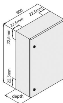
Pitch of holes for wall mounting (rear part of the rack)
