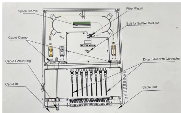
Diagram of MOTB-X16B
